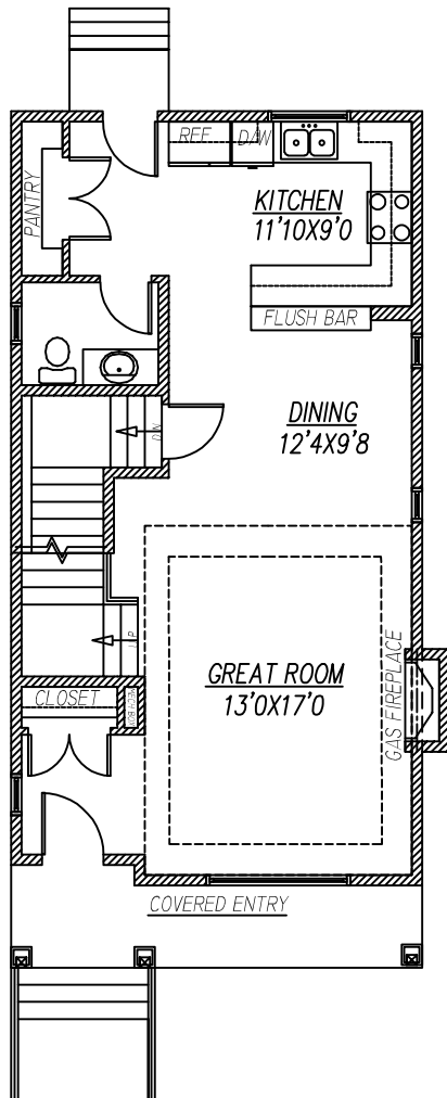
MAIN FLOOR PLAN 754 SQ. FT.
