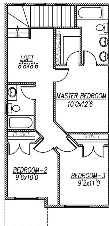
UPPER FLOOR PLAN 691 SQ. FT.
